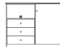
micro/fridge chest right 54" w x 24" d x 42" h microwave opening: 28.25" w x 20" d x 12" h refrigerator opening: 20" w x 20" d x 42.5" h 3 drawers with ball bearing glides recessed / vented back high pressure laminate top with solid wood edge, available with a false bottom drawer or no door
