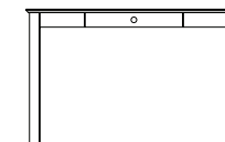
desk 48" w x 26" d x 30" h 1 drawer with ball bearing glides high pressure laminate top with solid wood edge, apron to floor: 26"
