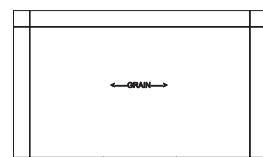
headboard full: 56" w x 1.5" d x 36" h queen: 62" w x 1.5" d x 36" h king: 78" w x 1.5" d x 36" h 1/8" grooved, wall hung, 1 panel
