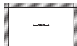
headboard two tone full: 56" w x 1.5" d x 36" h queen: 62" w x 1.5" d x 36" h king: 78" w x 1.5" d x 36" h 1/8" grooved, wall hung, 1 panel
